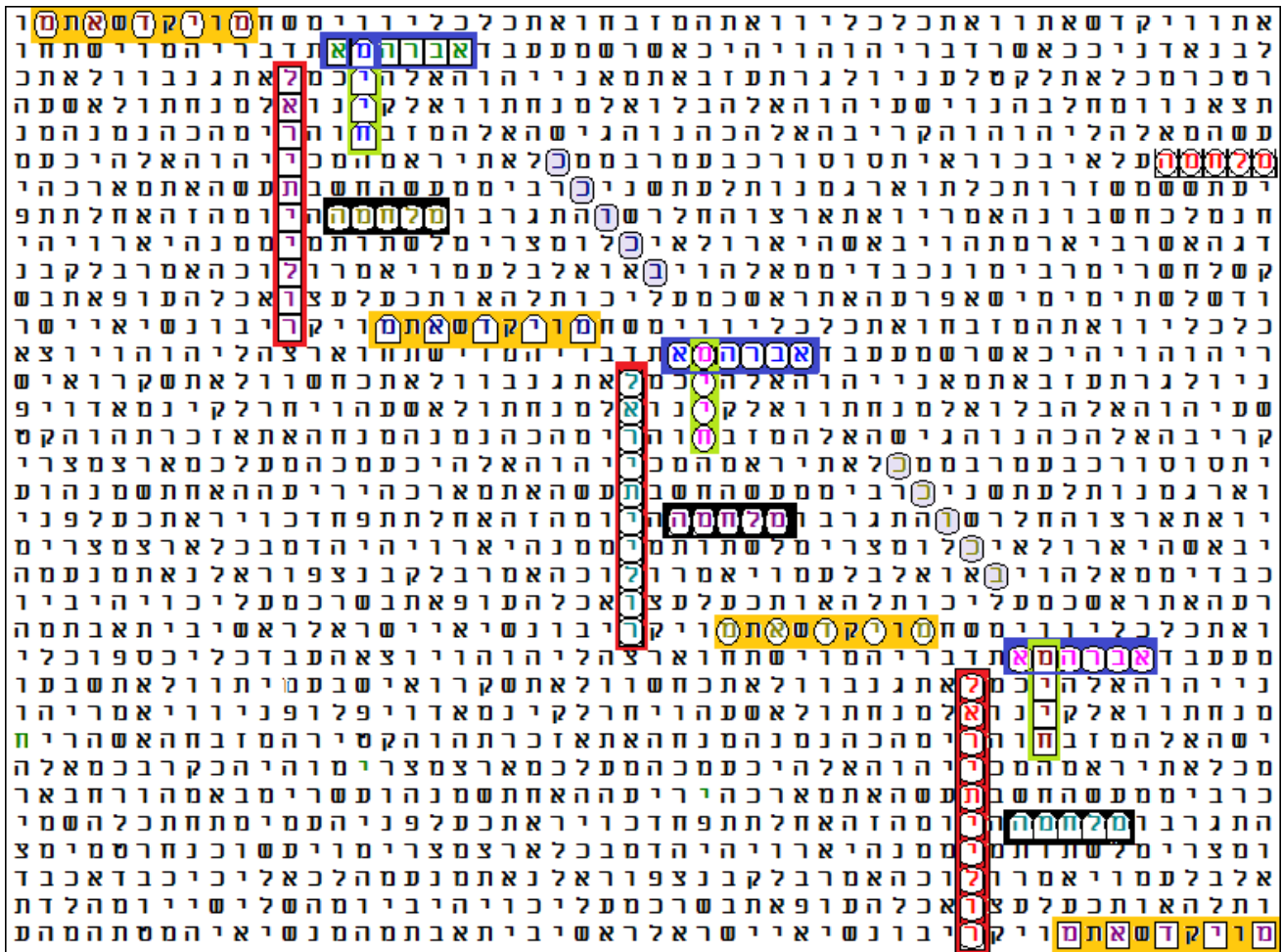
Figure E-20 above. Here, the matrix includes the terms MARS , LIKE A STAR , EBRAHIMI , LIFE and WAR . LIFE is at the absolute skip of LARRY TAYLOR and it intersects and shares a letter mem with EBRAHIMI .
