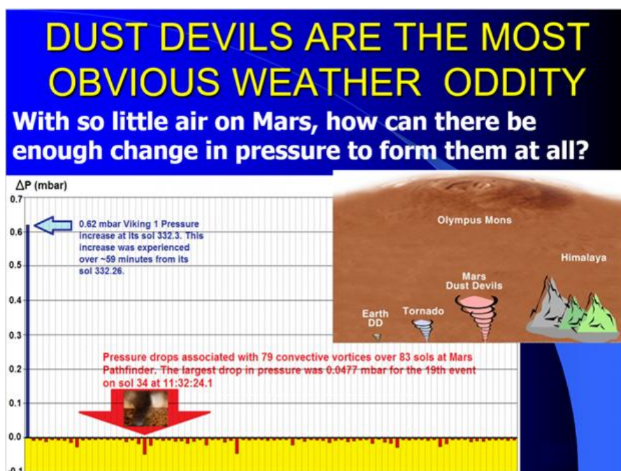
Figure 7-2 above. Relative magnitude of 0.62 mbar increases in pressure for Viking 1 at its sol (Martian day) 332.3 and pressure drops for 79 convective vortices/dust devils at Mars Pathfinder over its 83 sols. Source: Murphy, J. and Nelli, S., Mars Pathfinder Convective Vortices: Frequency of Occurrence (2002) http://tide.gsfc.nasa.gov/studies/Chen/proposals/IES/2002GL015214.pdf
