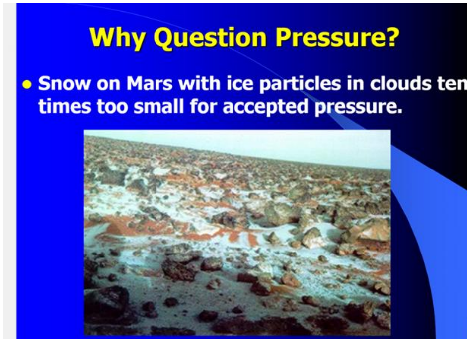
Figure 7-7 above: 2 \mu\text{m} ice particles survive on Mars because, in fact, the pressure is much higher than NASA has been telling us.
