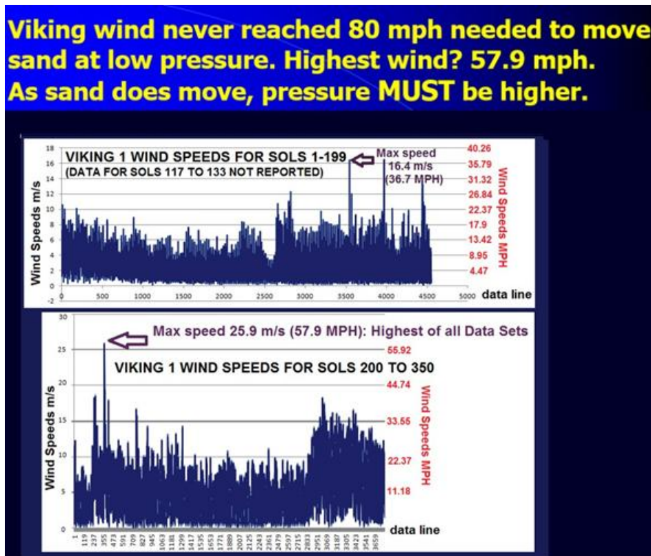
Figure 7-19 above: Wind speeds recorded at Viking 1 for its sols 1 to 116 and 134 to 350.
