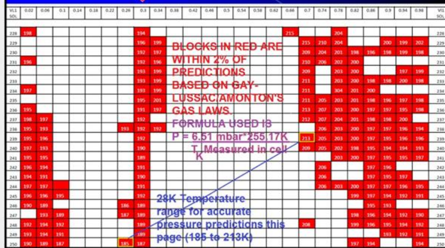
Figure 7-18 above: Sample of Annex F of Mars Correct: Critique of All NASA Mars Weather Data . Showing the times of day (for sols 228 through 250) when pressure predictions had less than a 2% difference from measured pressures at Viking 1. The formula used assumes that the pressure transducer is no longer in contact with the ambient atmosphere on Mars.
