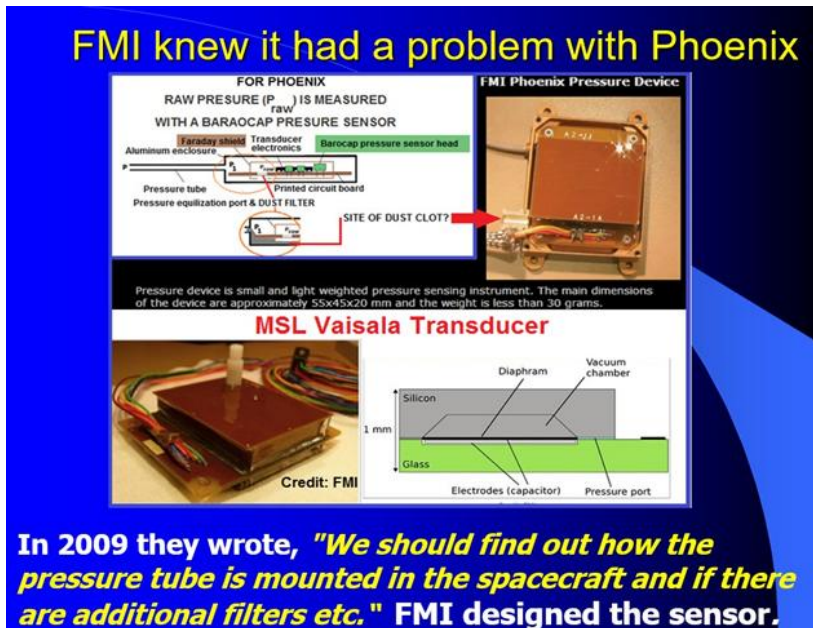
Figure 7-13: Phoenix and MSL pressure transducers.
