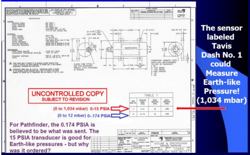
Figure 7-31 above: Reproduced from Tavis CAD Diagram 10484. For Mars Pathfinder, Tavis Dash No. 2 had a 0.174 PSIA limit (12 mbar), but Pathfinder Tavis Dash No. 1 had a 15 PSIA limit (1,034 mbar – best suited for Earth-like pressures). Source: Personal communication, Tavis Corporation 10/29/2009.
