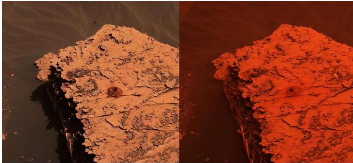
Figure 42 - Two images from the Mast Camera (Mastcam) on NASA's Curiosity rover depict the change in the color of light illuminating the Martian surface since a dust storm engulfed Gale Crater. The left image shows the "Duluth" drill site on Sol 2058 (May 21); the right image is from Sol 2084 (June 17). The cherry red color in the post-storm image is due to a few factors. One difference between the two images is exposure time: the dust over Curiosity creates a low-lighting condition that requires a longer exposure time for the camera. The pre-storm image had an exposure time of 7.3 milliseconds, which is normal for the rover; the later image had an exposure time that was 66 milliseconds -- or nine times longer. Credit NASA/JPL-Caltech/MSSS
