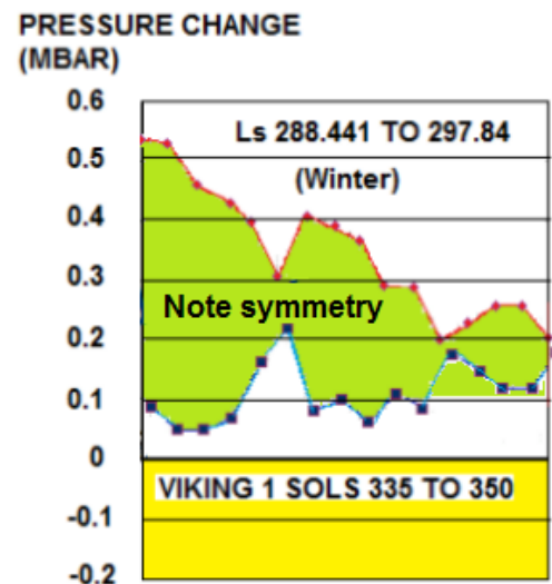
Figure 16F – Viking 1 Sols 335 to 350
