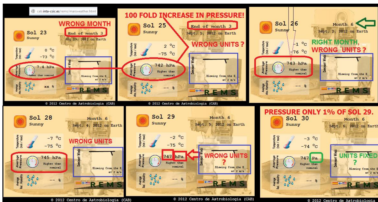
Figure 17A: REMS data confusion: For the first 2 months the Rover Environmental Monitoring Station (REMS) Team at the Centro de Astrobiología in Spain was confused about Martian month and pressure units. From September 1 to 5, 2012, they reported terrestrial-like pressures of over 740 hPa (mbar); then dropped back to similar numbers but with Pa. All winds were erroneously reported as 2 m/s (7.2 km/h).
