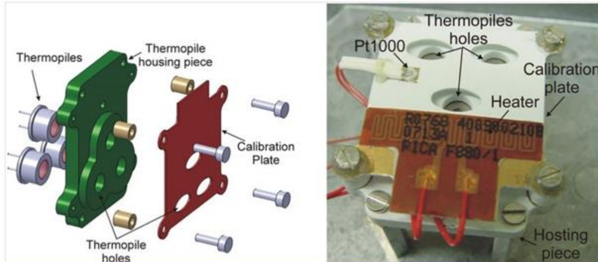
Figure 67 – The MSL Ground Temperature Sensor manufactured by the Institute for Physical High Technology, Jena, Germany.
